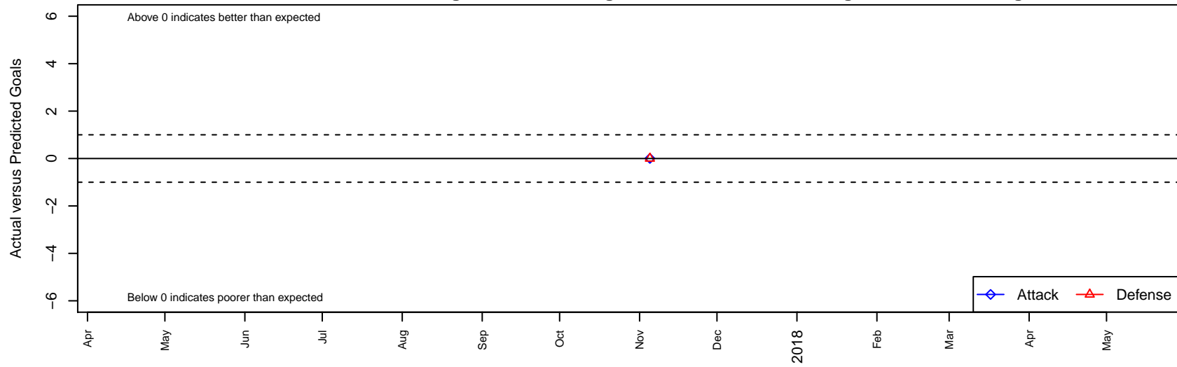
Los Angeles United FA USSDA B04 Dots are actual minus expected GF (blue circles) and GA (red triangles). Blue line is smoothed change in attack strength. Red is smoothed change in defense strength.
